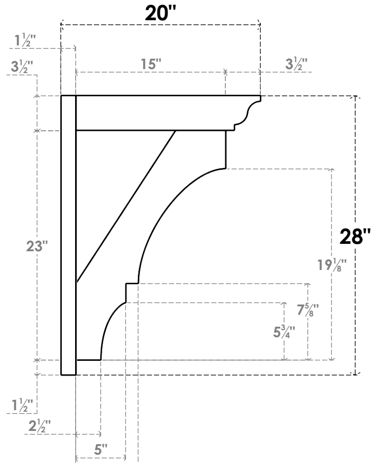
SIDE PROFILE
